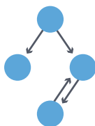
Unweighted
