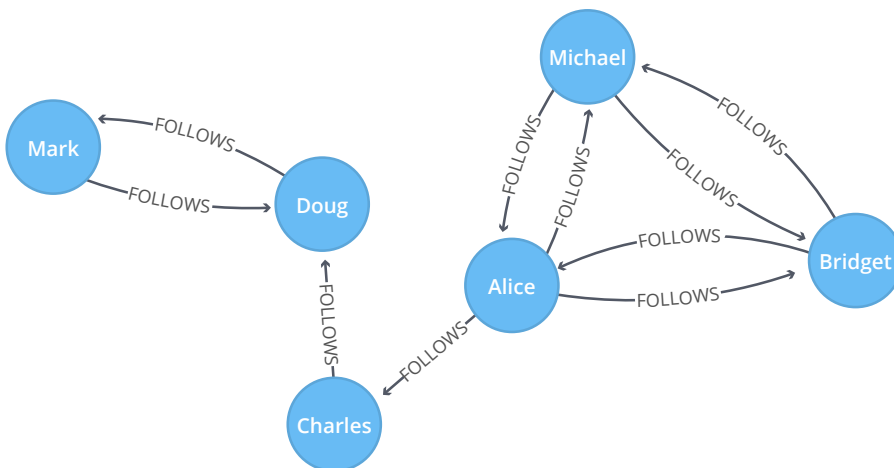
Graph Model
