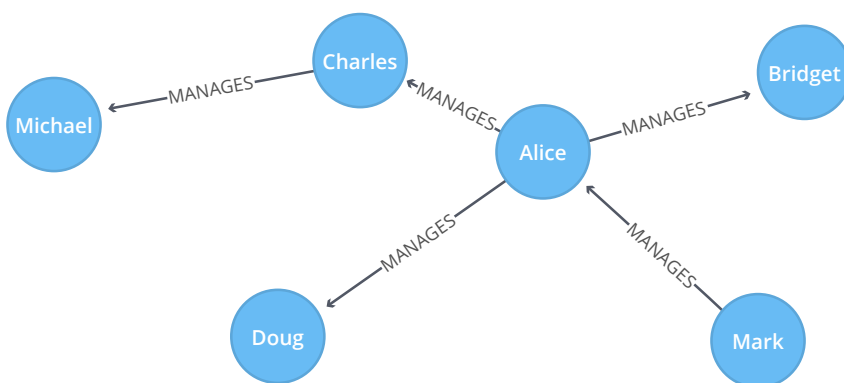
Graph Model
