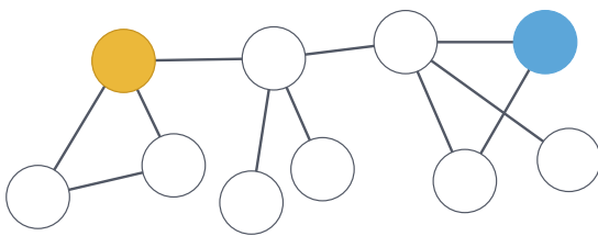
Pass 1
