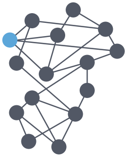
Step 0
