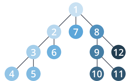
Depth-first search
