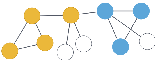
Pass 1
