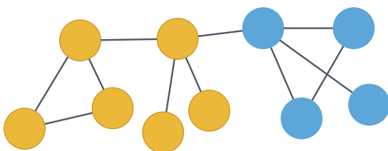
Pass 2
