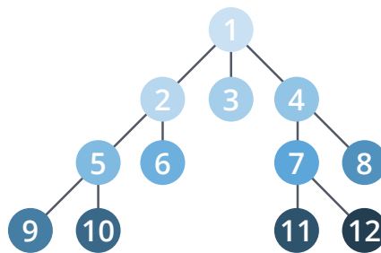
Breadth-first search
